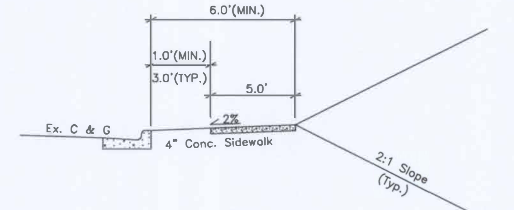
Typical Section (NTS)
