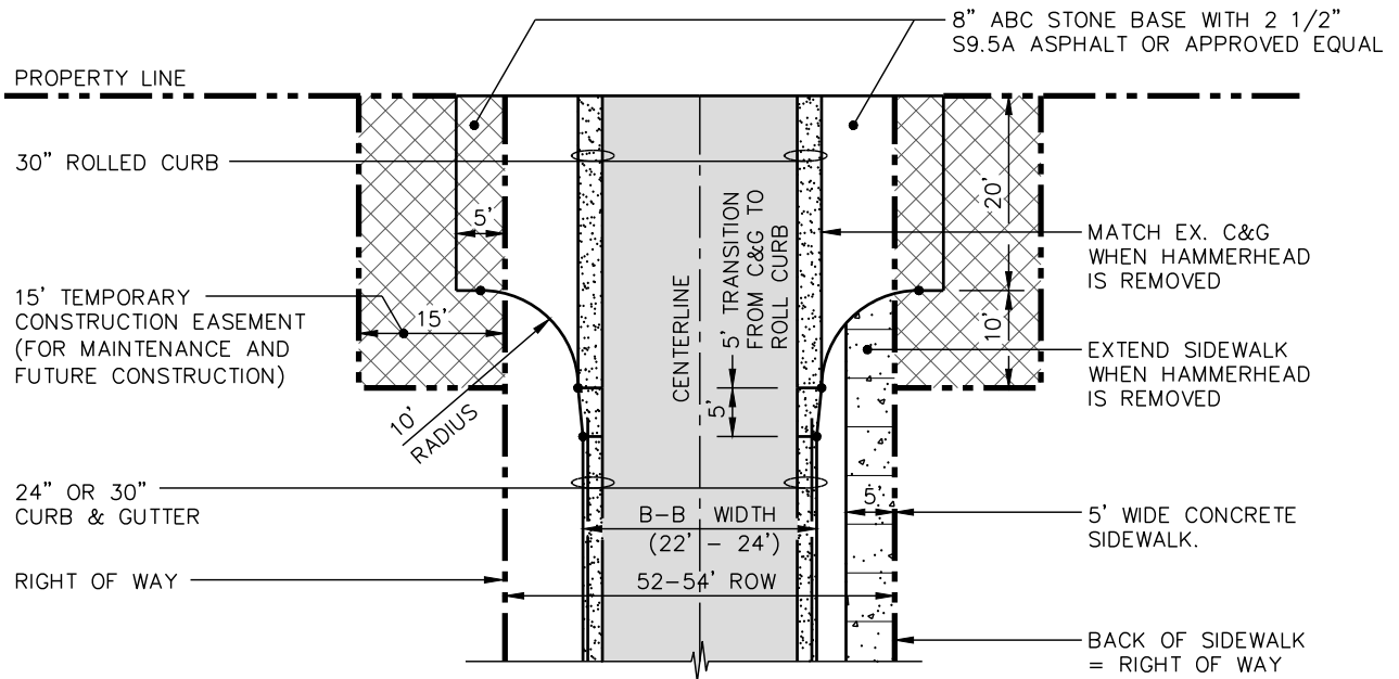
52-54' RIGHT-OF-WAY
