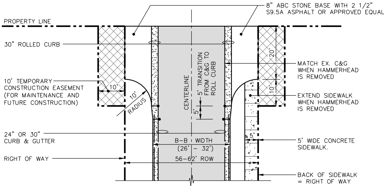
56-62' RIGHT-OF-WAY
