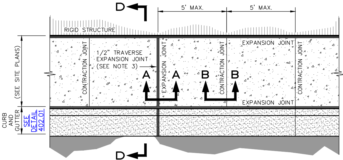
SIDEWALK abutting CURB / RIGID STRUCTURE
