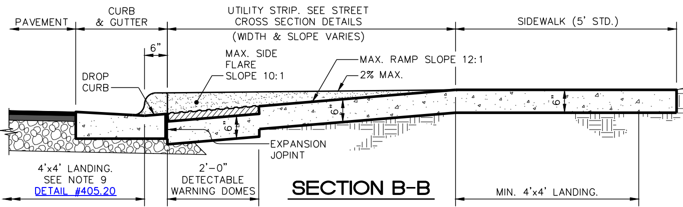
CURB ELEVATION
