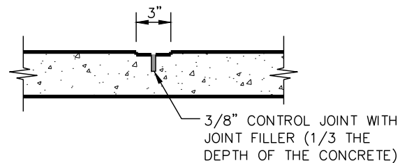
SECTION B-B CONTROL JOINT
