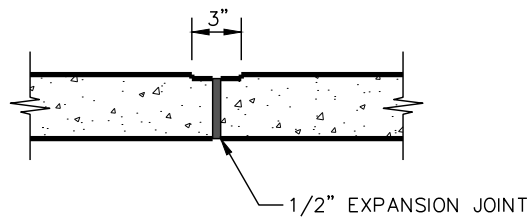
SECTION A-A EXPANSION JOINT
