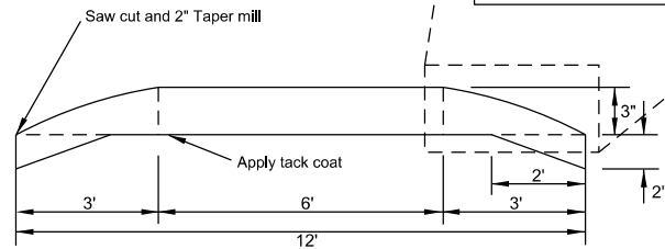
SECTION B-B 1V = 4H
