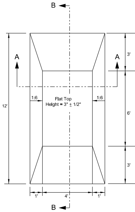
SPEED CUSHION PLAN VIEW
