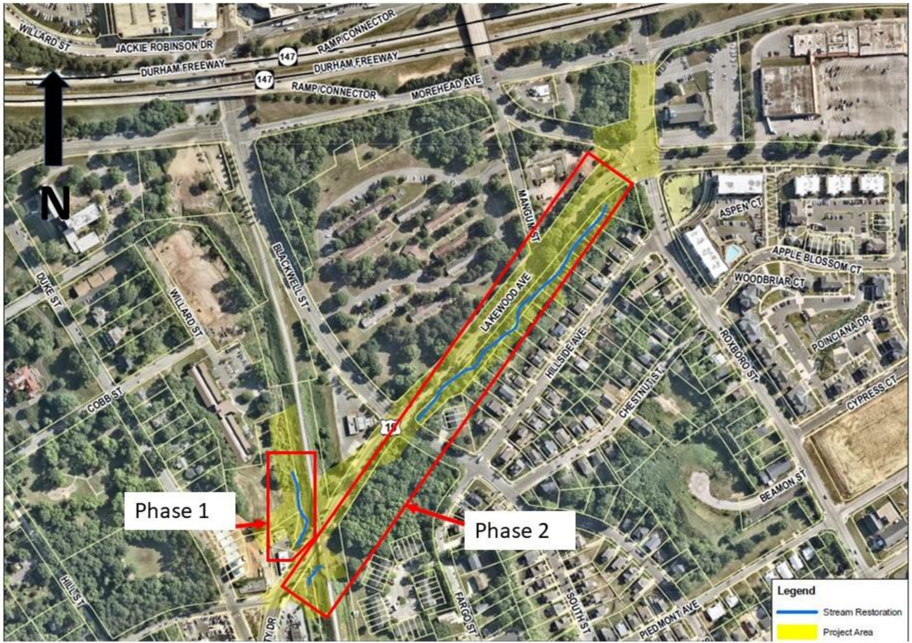
Lakewood Ave Stream Stabilization and Enhancement Map, Phase 1 and Phase 2
